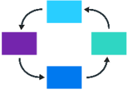
Iterative
