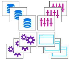
Microservices + APIs
