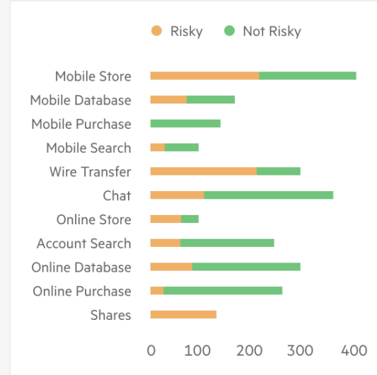
Features Per Application Modules - By Team
